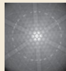
CBED diffraction image of the corresponding area in the Si crystal.
