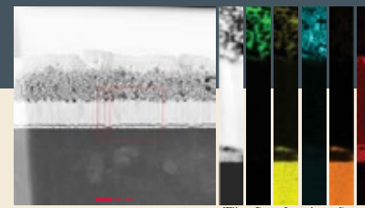
Au Catalysts HAADF STEM + EDX, STEM EDX drift-corrected mapping of layers. The mapped region is 25x190 pixels where 1 pixel is 4x4 nm. We find signals from the 5 elements mapped above.
